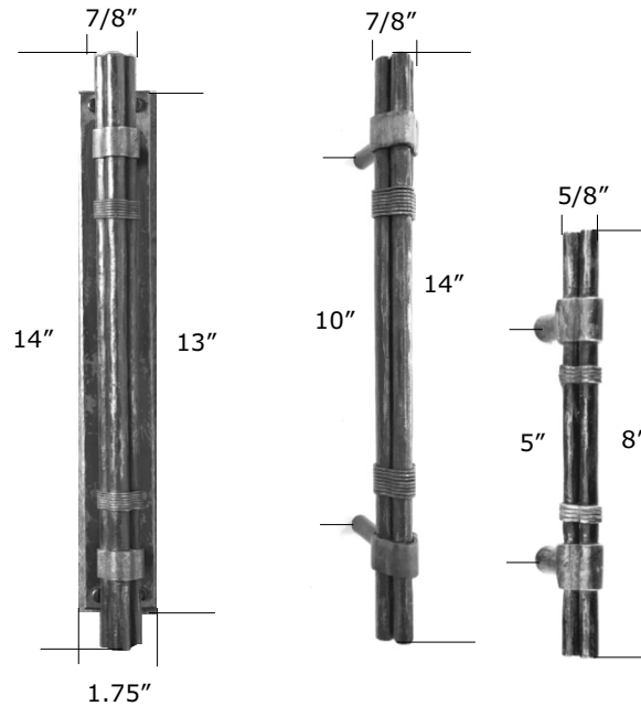
HP706-ESC HP706 HP706S (3.5" projection) (3 1/8" projection) (1 3/4" projection)
