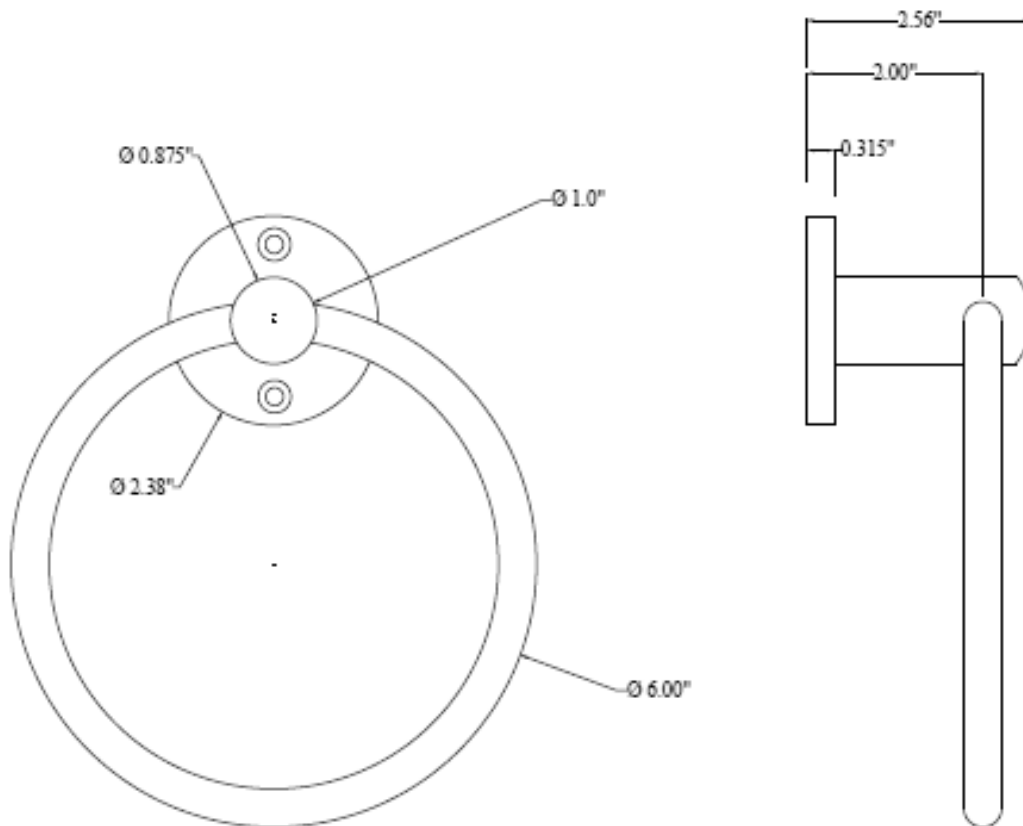
Bronze BT621 Round Towel Ring
